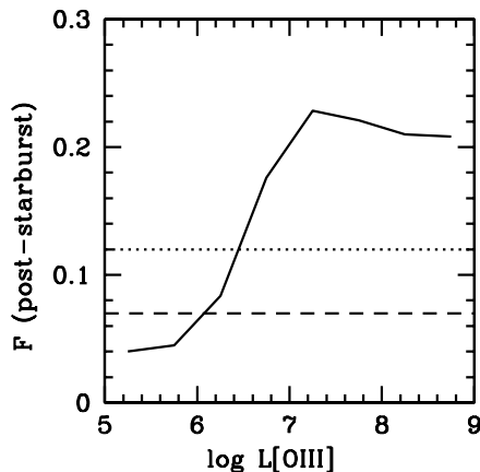
Figure 18: The fraction F of AGN with H\delta_A values that are displaced by more than 3\sigma above the locus of star-forming galaxies is plotted as a function of \log L[\text{OIII}] . The dashed line indicates the fraction of such systems in the subsample of normal massive galaxies. The dotted line indicates the fraction of such systems in the subsample of normal massive galaxies with D_n(4000) < 1.6 .
